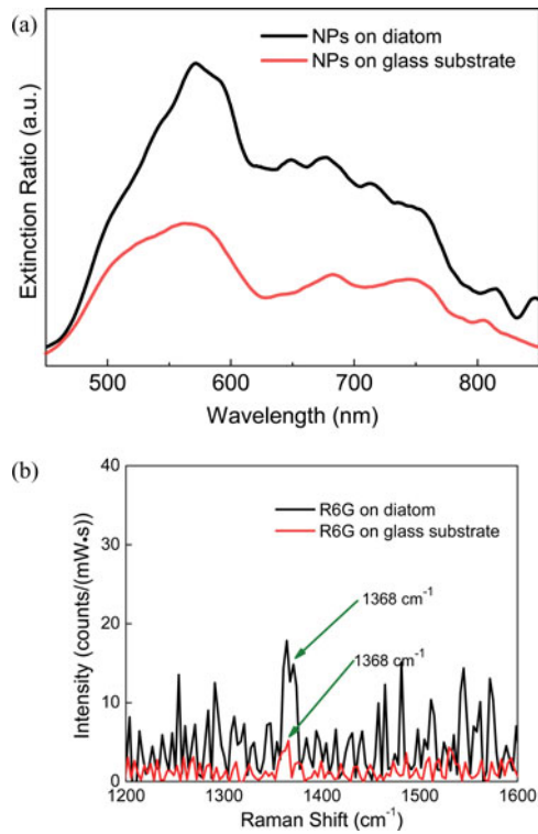
Fig. 6. (a) Measured extinction spectra of NPs on a diatom frustule (black) and Ag NPs on a glass substrate (red). (b) Raman spectra of 5 mM R6G on diatom (black) and glass substrate (red). During the Raman measurement, the excitation power was set at 1.2 mW and integration time was 5 s.
