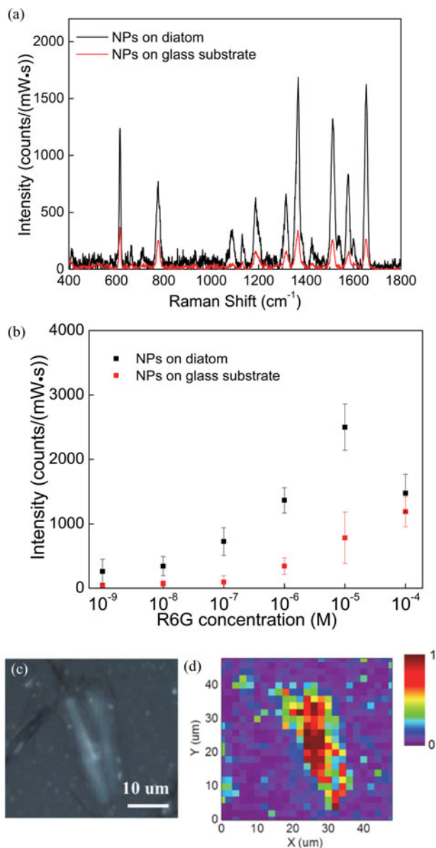
Fig. 3. (a) SERS spectra of 1 \mu\text{M} R6G coated on Ag NPs-on-diatom (black) and Ag NPs-on-glass (red). (b) Intensities of Raman band at 1368 \text{cm}^{-1} for different R6G concentrations. (c) Optical image of the sensing area scanned for SERS enhancement and (d) mapping of Raman signal intensity at 1368 \text{cm}^{-1} . During the measurement, the excitation power was set at 1.2 mW and integration time was 1 s.
