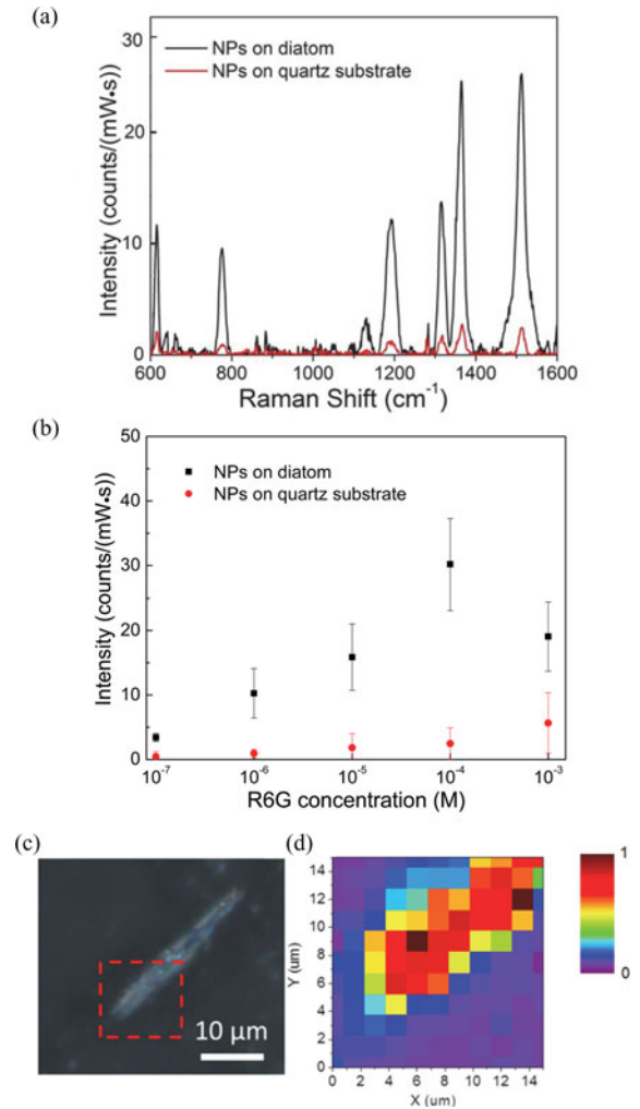
Fig. 5. (a) SERS spectra of 100\ \mu\text{M} R6G coated on Ag NPs-on-diatom (black) and Ag NPs-on-quartz (red), (b) Intensities of Raman band 1368\text{ cm}^{-1} for different R6G concentrations. (c) Optical image of the area scanned for SERS measurement, and (d) map of Raman signal intensity at 1368\text{ cm}^{-1} . During the measurement, the integration time was 60 s and the grating groove density was set at 300/\text{mm} . The excitation power was 2.1 mW.
